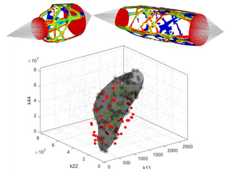
Fig. 2: Top: Optimized components Bottom: Space of feasible component properties
