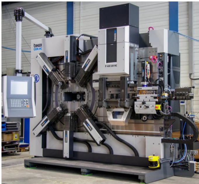
Figure 1, GRM NC Stamping machine
