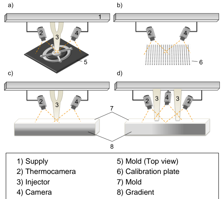
Figure 1: Schematic structure of the casting system with thermo-stereo camera system a) in the casting machine, b) for the calibration, c) Y-variant with horizontal and d) II-variant with vertical gradient
